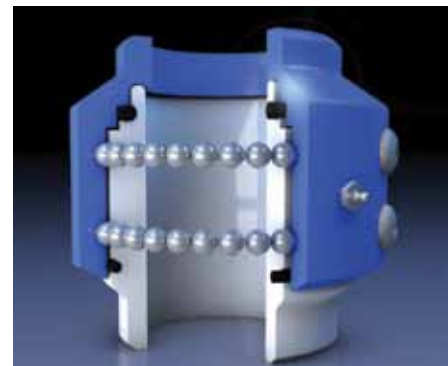
Cast High-Pressure Steel (Main Seal has Teflon® Back-up Ring)
