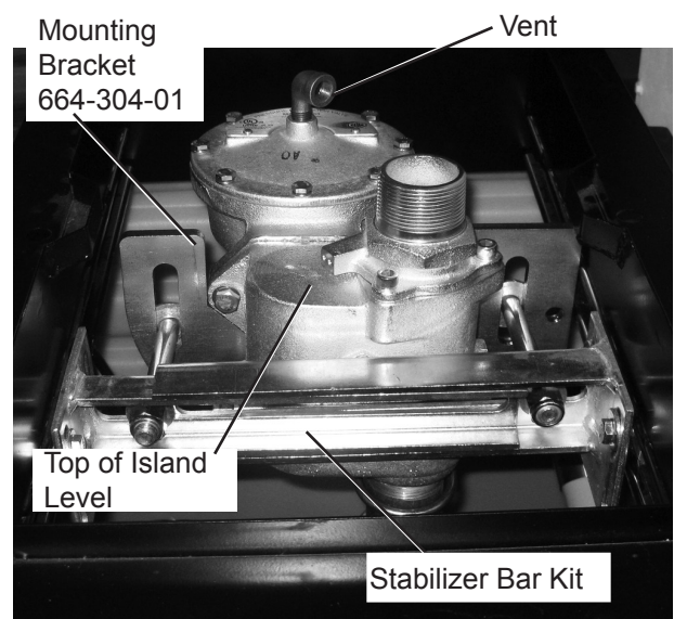
Figure 2: 664 Valve Installation
