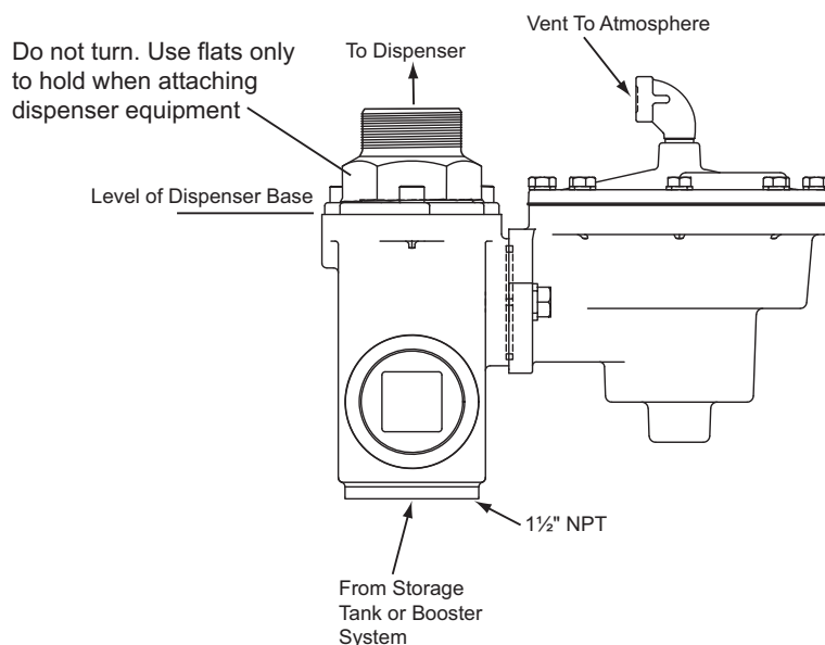
Figure 1: 664 Valve Side View
